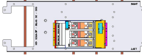
SILAS Gr. 00 (160 A)
